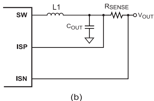
Figure 2—Current Sensing Methods
